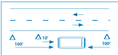
ONE-WAY TRAFFIC OR DIVIDED HIGHWAY
