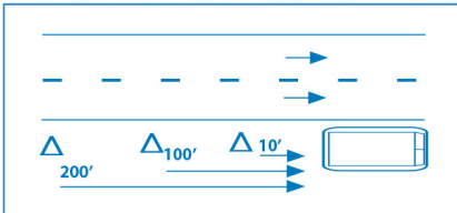
CURVE OR HILL CREST
